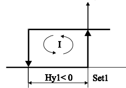
Direct action (dehumidification) with negative differential
