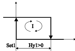
Inverse action (humidification) with differential positive
