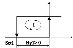
Direct action (dehumidification) with positive differential
