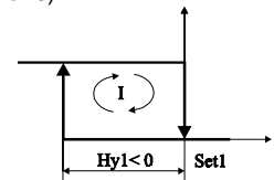
Inverse action (humidification) with negative differential
